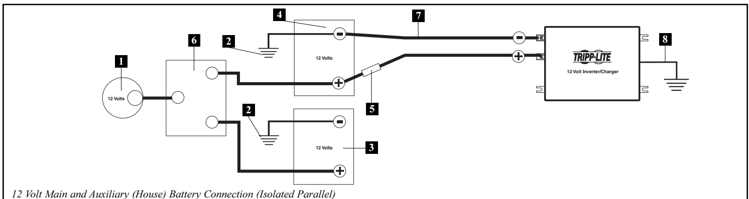
12 Volt Main and Auxiliary (House) Battery Connection (Isolated Parallel)
